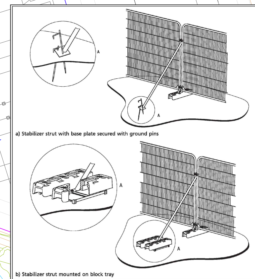
Tree Protection Fencing Specification
